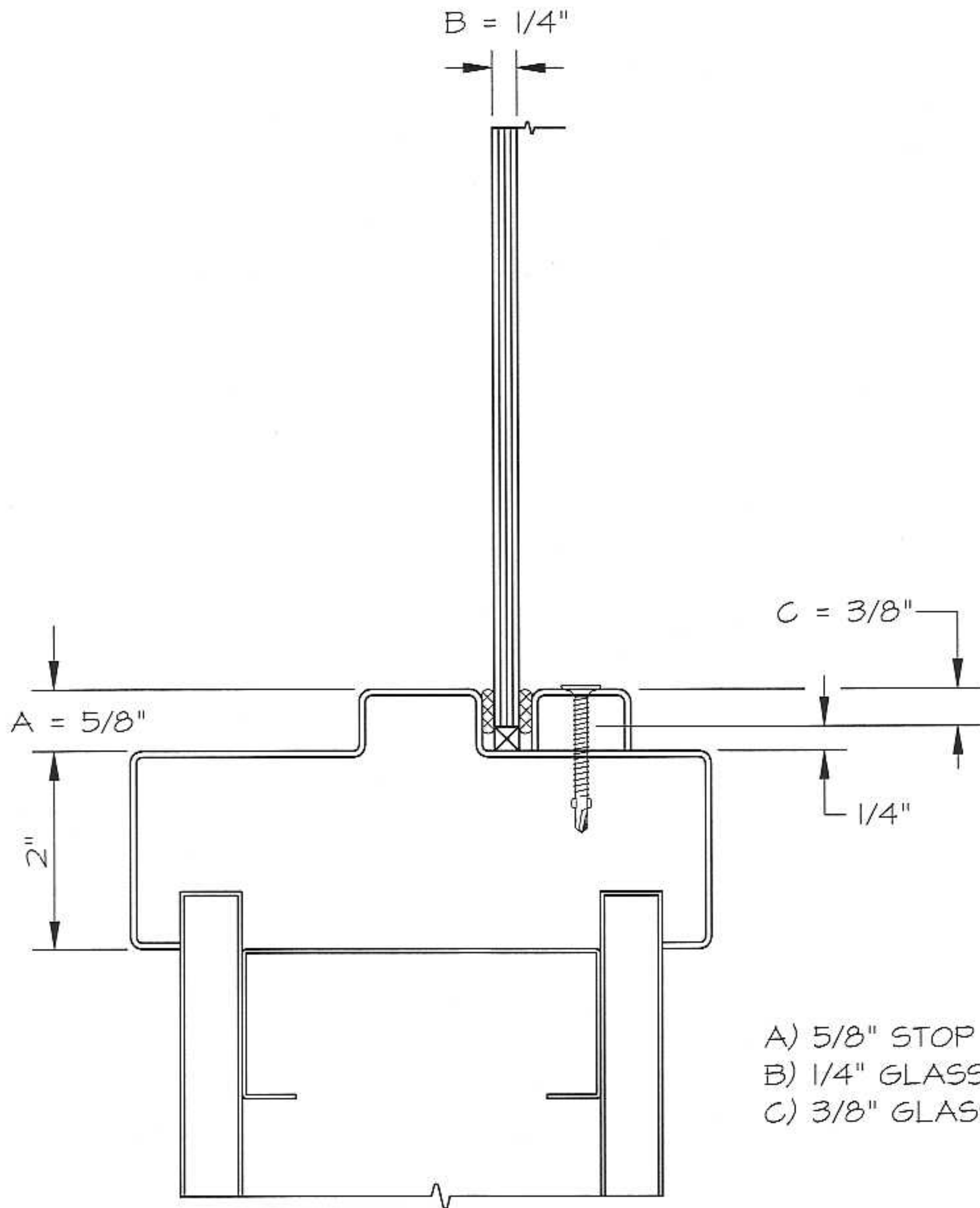
HOLLOW METAL FRAME 45/60 MINUTE SUPERLITE-1
